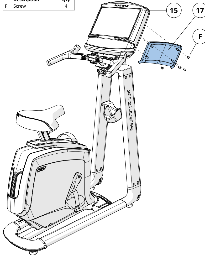
Hardware For Step 6
