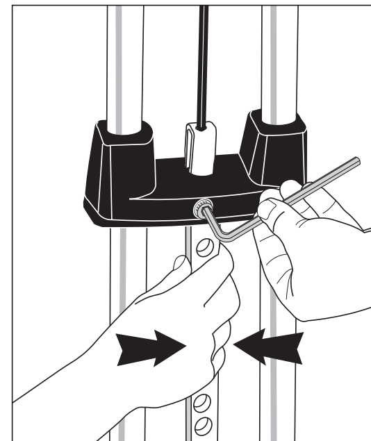
D Once the Selector Stem is centered, retighten the socket cap bolt securely.
