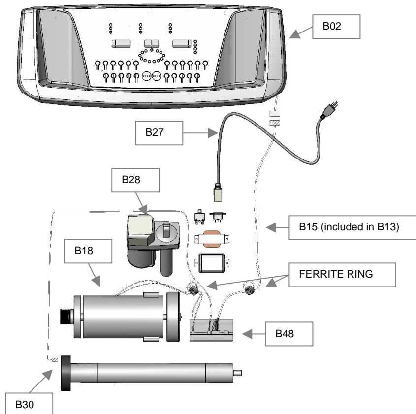
Figure 1 Electrical components and their connections (numbering refers to spare part diagram)
