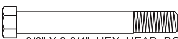
3/8" X 2-3/4" HEX HEAD BOLT(65)
