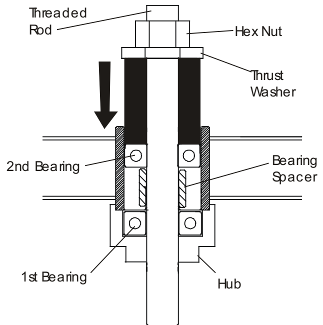
PUSH IN □ OUT 1st BEARING
