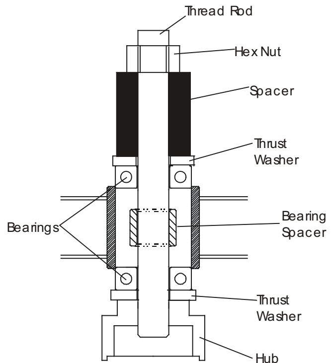
SET UP THE PULLER FOR PRESSING IN BEARINGS
