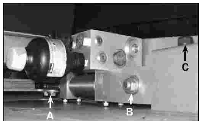
Figure 4: Hydraulic Cylinder bolt locations:
