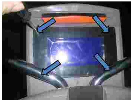
Step 2: Use a Phillip screw driver to open fix console main PCB 4 bolts on the upper console plastic cover.
