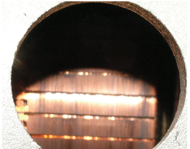
Cleaned Communtator
