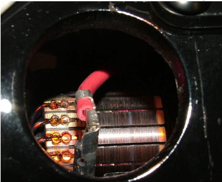
Cleaned Communtator
