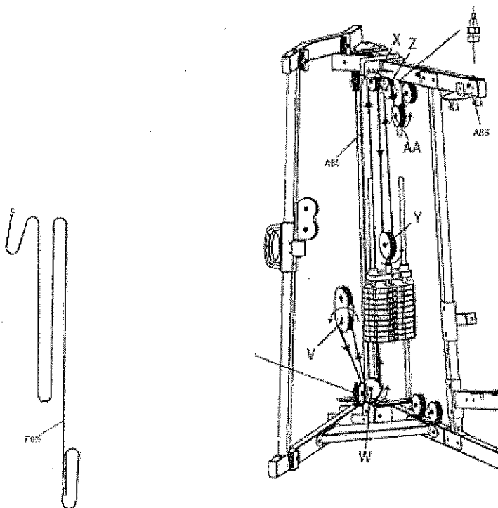
Cable 4 – F05 – "Weight stack cable/main pulley cable"
