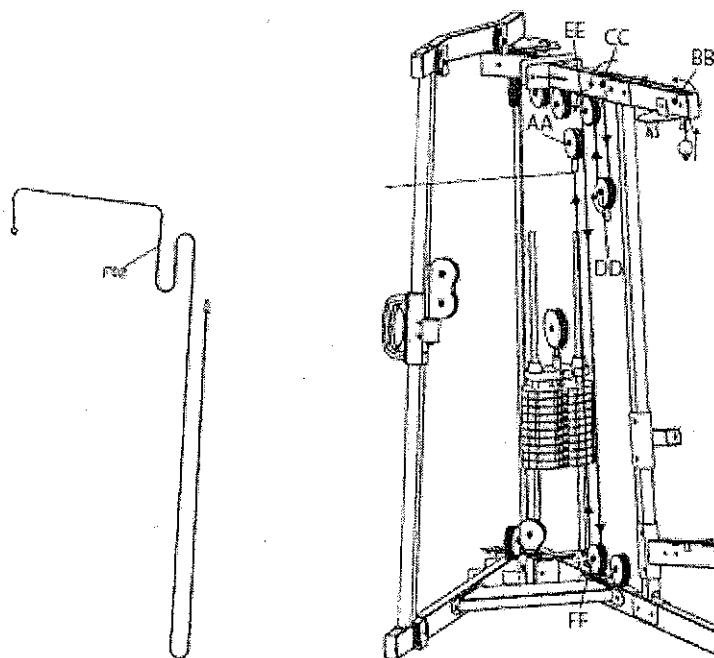
Cable 5 – F02 – "Lat/Pulldown Cable"
